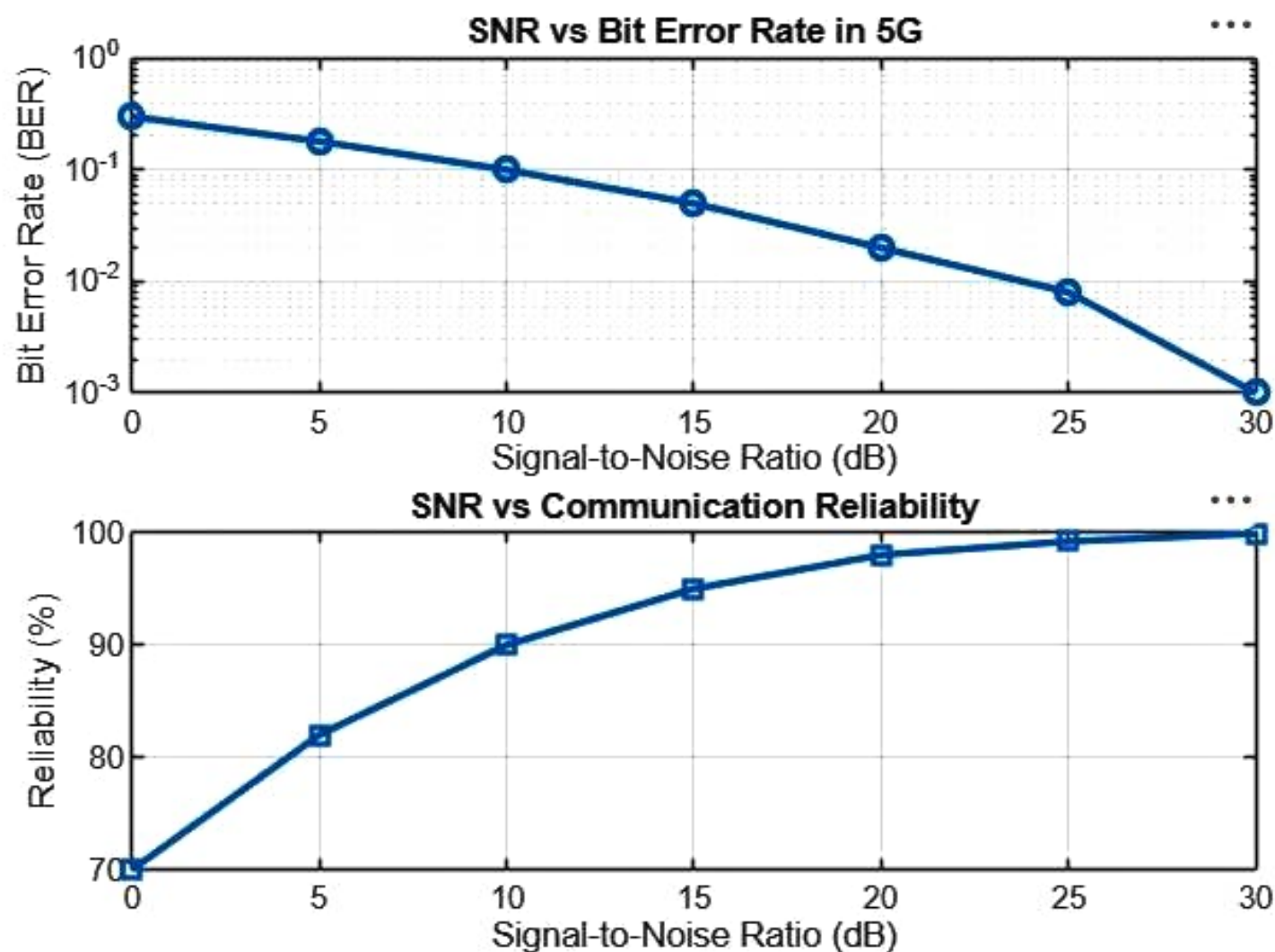
Command Window
